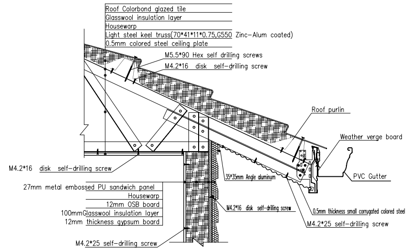
Details for roof and eave
