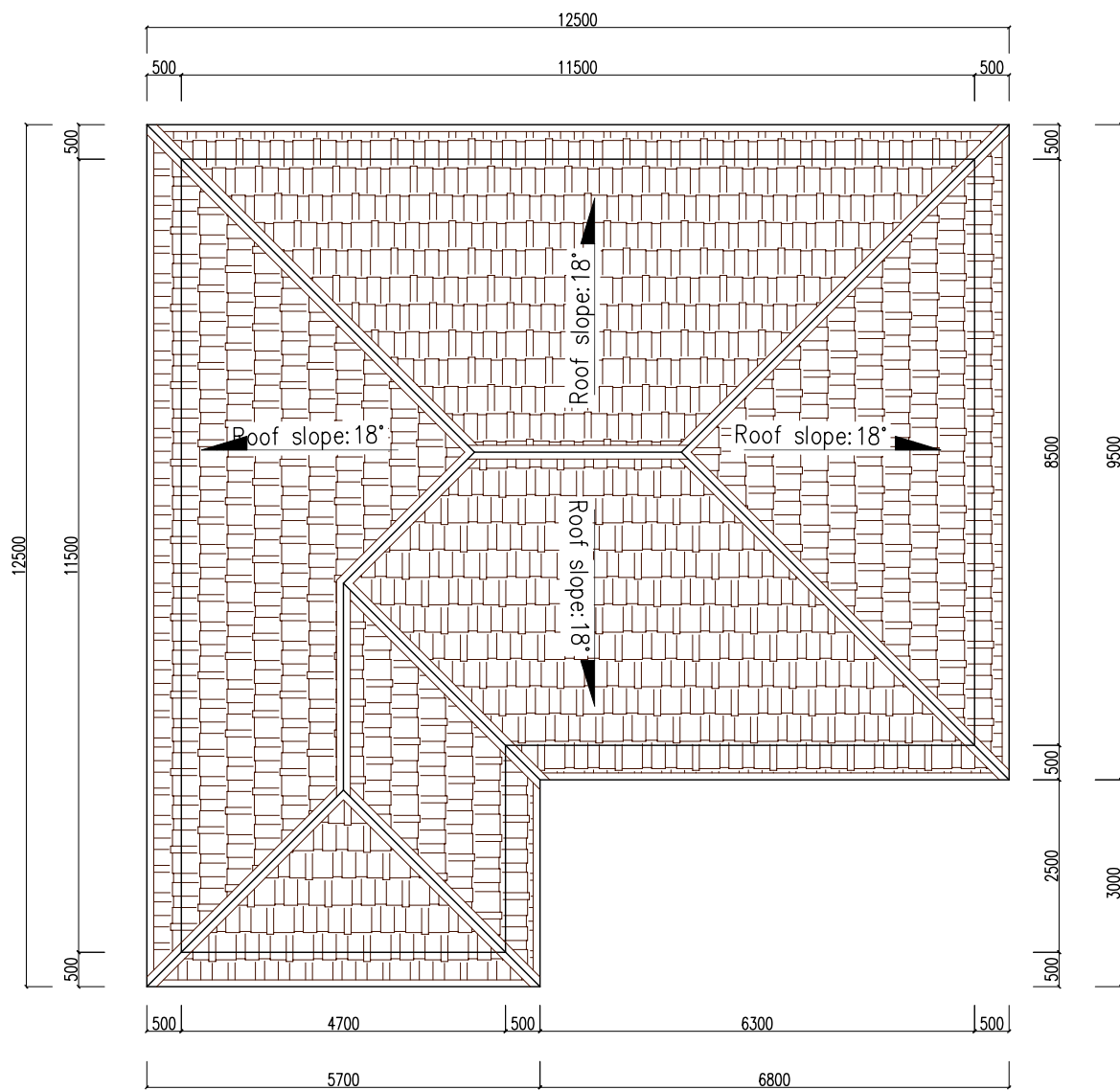
Layout for roof plan
