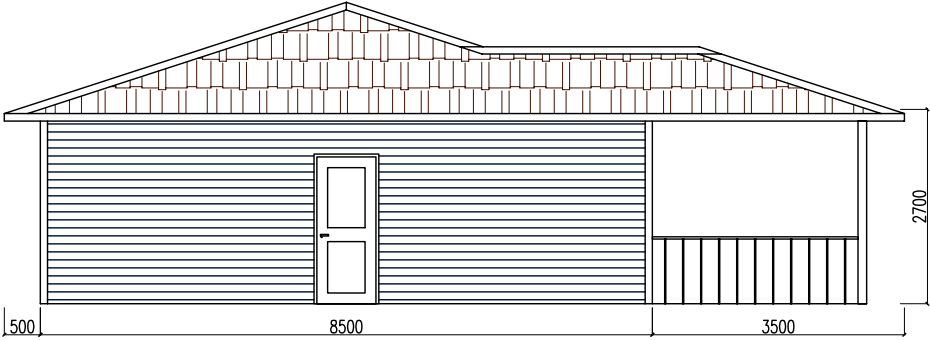
West Elevation
