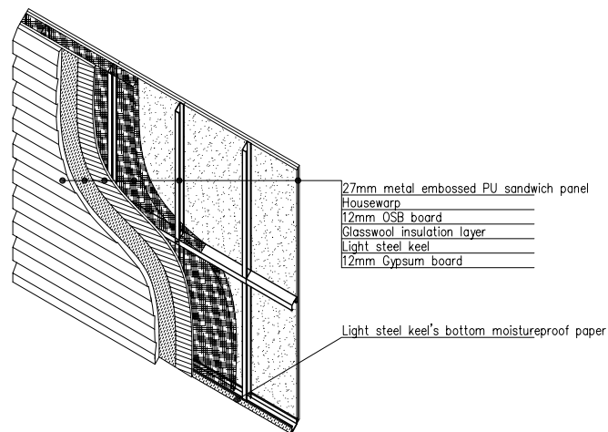
Details for outside wall
