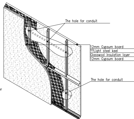
Details for inside wall
