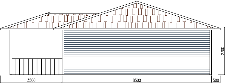
East Elevation
