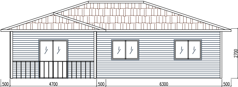
South Elevation
