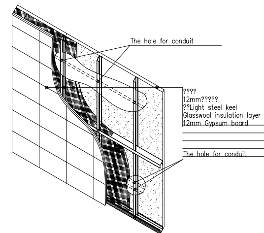
The details for toilet and kitchen wall
