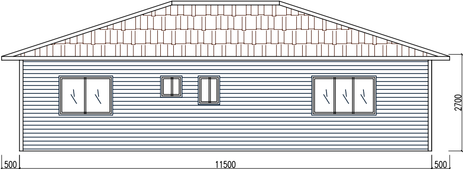
North Elevation
